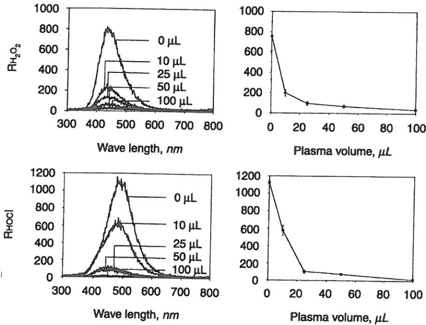
Fig. 2. Typical emission spectra of the chemiluminescence (CL) of a test mixture containing H_2O_2 and luminol for reference H_2O_2 ( R_{H_2O_2} ), HOCl, and luminol for reference HOCl ( R_{HOCl} ) and different volumes of plasma or [phosphate-buffered saline (PBS)] obtained from a healthy control. Increased plasma volume (from 0 to 100 \mu\text{L} ) added to the test mixture could lower both R_{H_2O_2} and R_{HOCl} counts. Mean change of R_{H_2O_2} and R_{HOCl} counts with different plasma volume added to the test mixture was displayed in the right panels.
