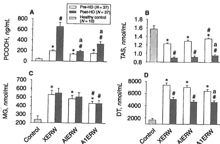
Fig. 6. Effects of hemodialysis (HD) and electrolyzed reduced water (ERW) supplementation on PCOOH (A), total antioxidant status (TAS) (B), methylguanidine (MG) (C), and dityrosine (DT) (D) in plasma obtained from 37 end-stage renal disease (ESRD) patients. The levels in PCOOH, MG, and DT of prehemodialysis plasma in 37 ESRD patients without ERW treatment (XERW) were higher than those in 10 healthy control subjects. A significant decrease in TAS of prehemodialysis plasma was found in ESRD patients. When compared to prehemodialysis value, the posthemodialysis plasma had significantly elevated PCOOH levels and marginally increased MG and decreased TAS and DT values. Initial ERW (A1ERW) supplementation significantly reduced PCOOH levels, but did not significantly affect TAS, MG, and DT values. However, 1-month ERW (A1MERW) supplementation mildly restored TAS ability in posthemodialysis plasma and consequently mildly reduced PCOOH, MG, and DT levels in posthemodialysis plasma. The level of PCOOH in posthemodialysis plasma after 1-month ERW treatment was higher than that after initial ERW treatment possibly by a dietary factor. Note that a marginally increased TAS, and a decreased MG was found in prehemodialysis plasma after 1-month ERW treatment. * P < 0.05 the prehemodialysis values of ESRD plasma vs. the values of healthy control plasma. # P < 0.05 the posthemodialysis values vs. the prehemodialysis value of the respective group. ^aP < 0.05 when compared to the value of ESRD plasma without ERW (XERW) administration.
