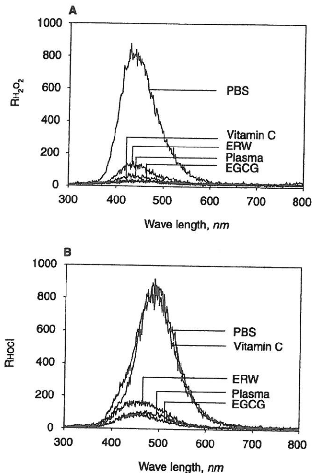
Fig. 3. Typical emission spectra of the reference H_2O_2 ( R_{H_2O_2} ) (A) and reference HOCl ( R_{HOCl} ) (B) counts with various kinds of antioxidants [vitamin C, epigallocatechin-3-gallate (EGCG), and electrolyzed reduced water (ERW)], plasma from healthy subjects and phosphate-buffered saline (PBS) are displayed. Vitamin C, ERW, plasma, and EGCG significantly reduced R_{H_2O_2} counts, whereas ERW, plasma, and EGCG, but not vitamin C, decreased R_{HOCl} counts.
