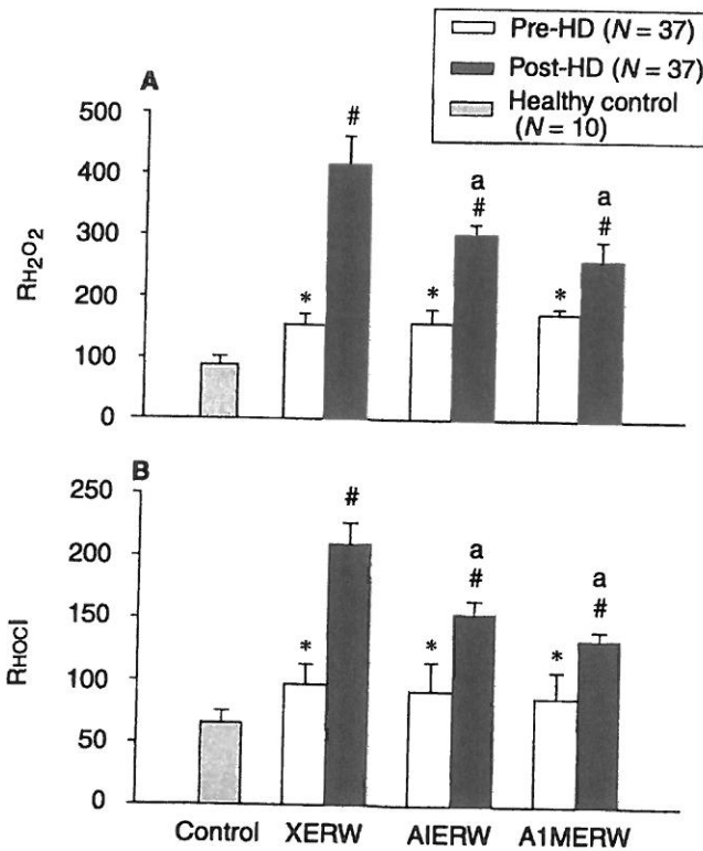
Fig. 5. Effects of hemodialysis (HD) and electrolyzed reduced water (ERW) supplement on reference H_2O_2 ( RH_2O_2 ) (A), and reference HOCl ( RHocl ) (B) counts in plasma obtained from 37 end-stage renal disease (ESRD) patients. The levels of RH_2O_2 and RHocl of prehemodialysis plasma in 37 ESRD patients were higher than those in 10 healthy control subjects. The posthemodialysis plasma had elevated RH_2O_2 and RHocl . However, after initial (A1ERW) and 1-month ERW (A1MERW) supplementation resulted in augmented reactive oxygen species (ROS) scavenging activity for both H_2O_2 and HOCl, as shown by the marked reduction of RH_2O_2 and RHocl . * P < 0.05 the prehemodialysis values of ESRD plasma vs. the values of healthy control plasma; # P < 0.05 the posthemodialysis values vs. the prehemodialysis value of the respective group. a P < 0.05 when compared to the value of ESRD plasma without ERW (XERW) administration.
